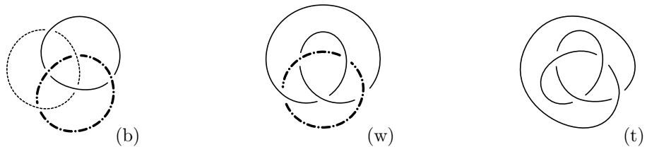
FIGURE 1. From Borromean rings to the Whitehead link and then to the trefoil knot
