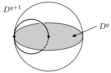
FIGURE 1. To the construction of the Hudson torus
