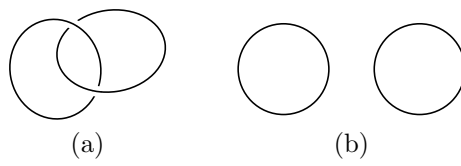
FIGURE 1. The Hopf link and the trivial link
