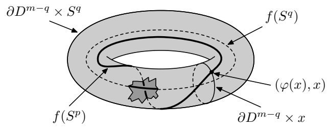
FIGURE 1. A link with prescribed linking coefficient
