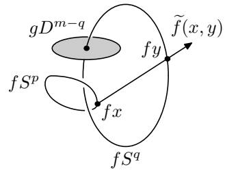
FIGURE 1. The Gauss map \tilde{f} and the disk gD^{m-q}
